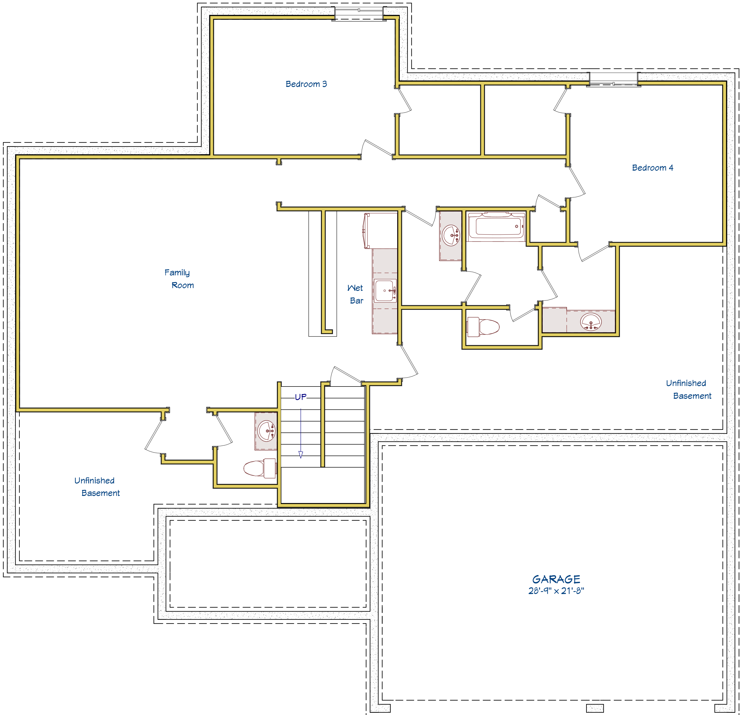
Foundation
